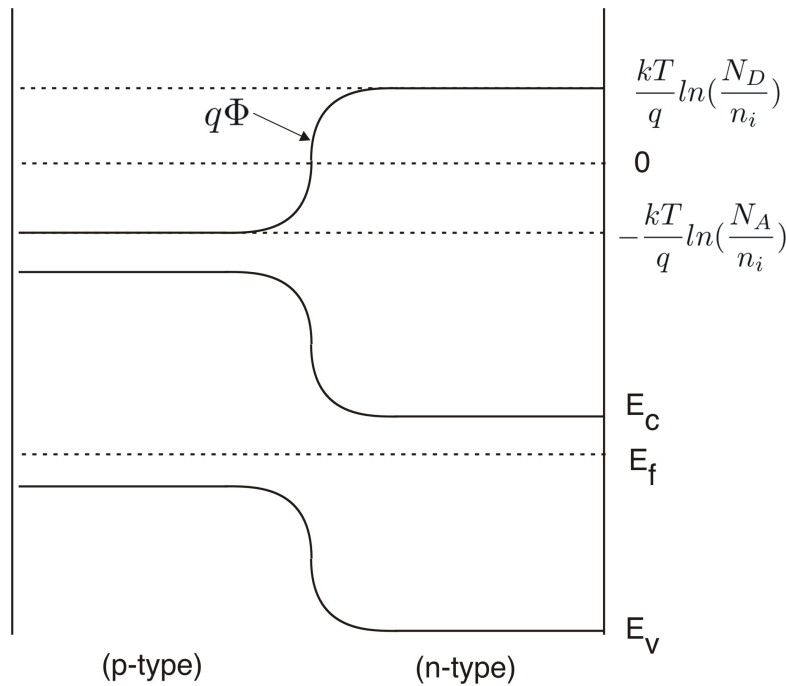
Figure 2-8. Neutral Contacts.
